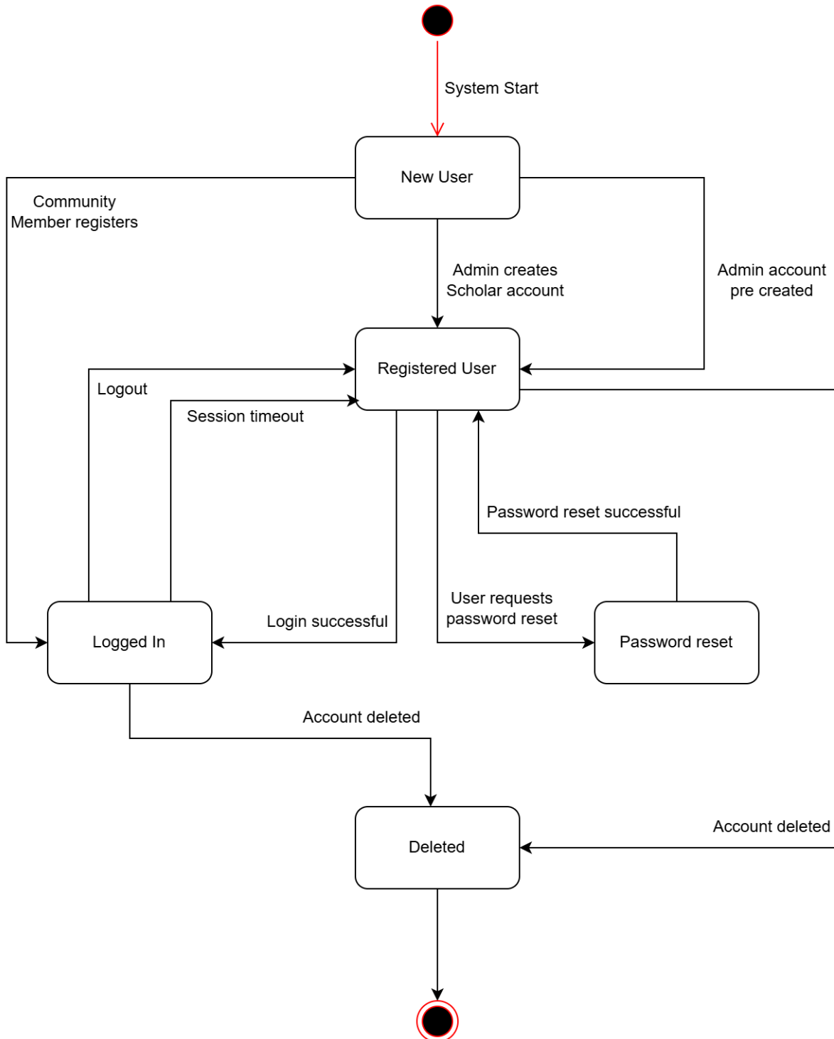
Figure 15 User Account State Diagram
