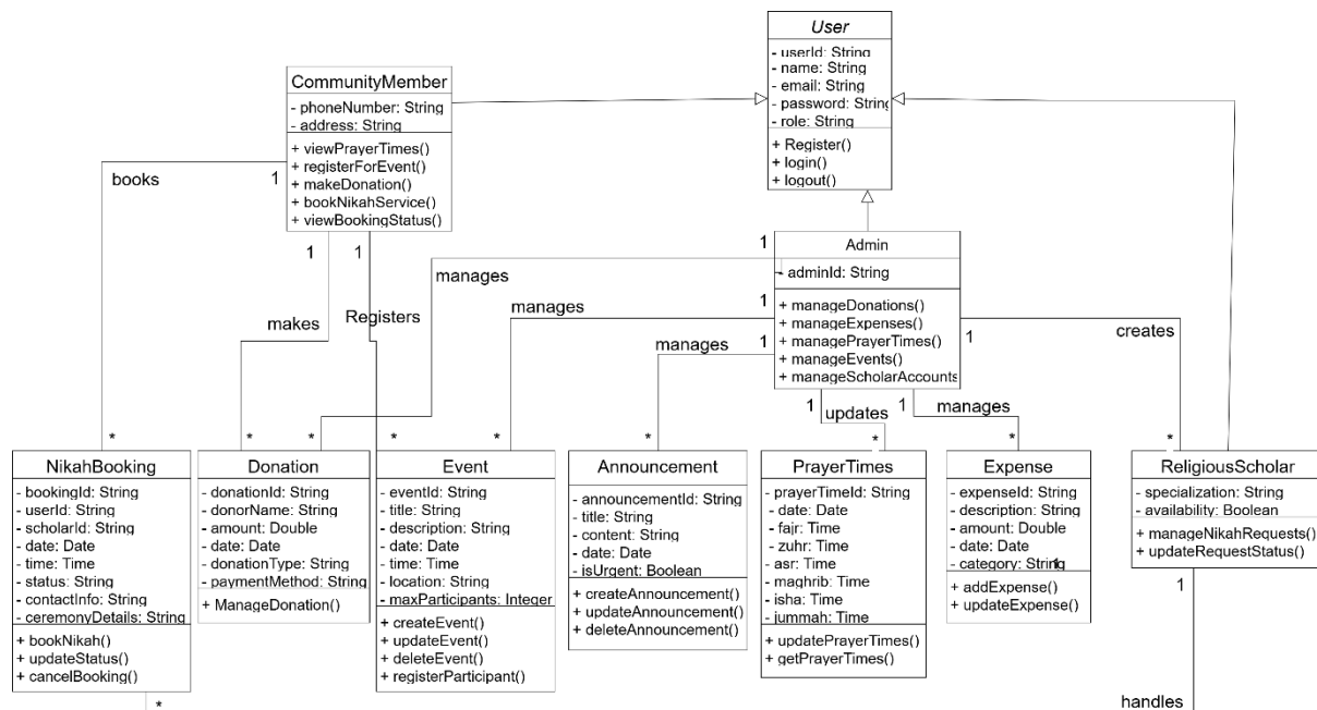
Figure 10 Class diagram
