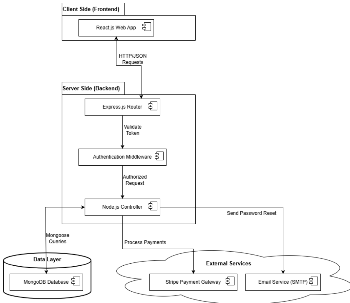
Figure 18 Architectural diagram
