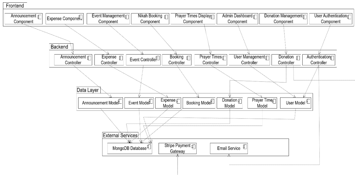
Figure 19 Component diagram
