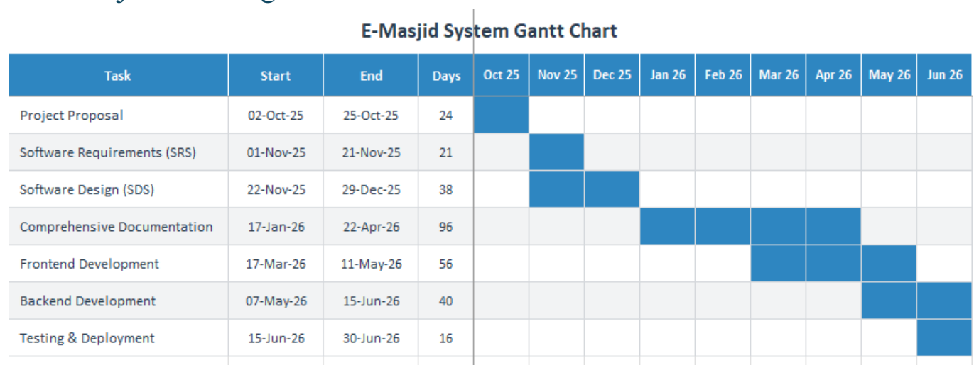
Figure 1 Gantt chart
